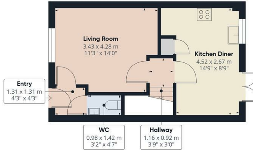
Floor 0
