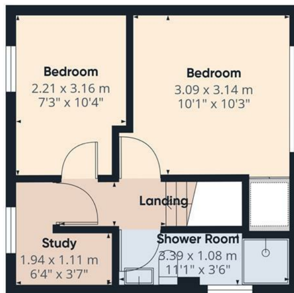
Floor 1
