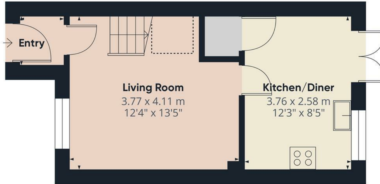
Floor 0
