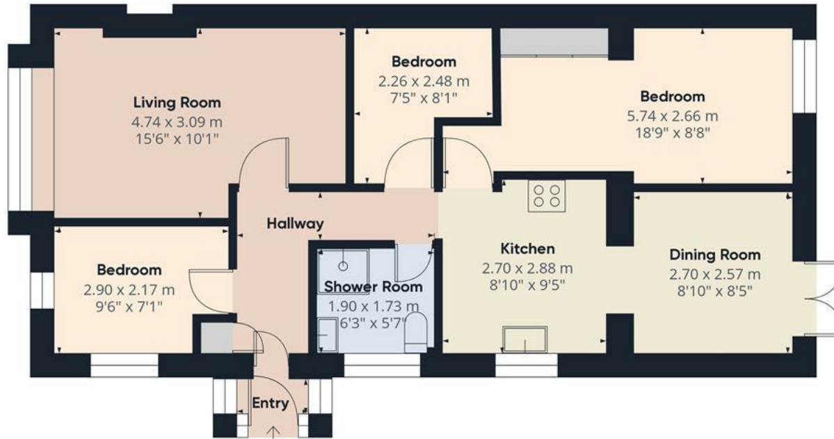
Floor 0 Building 1
