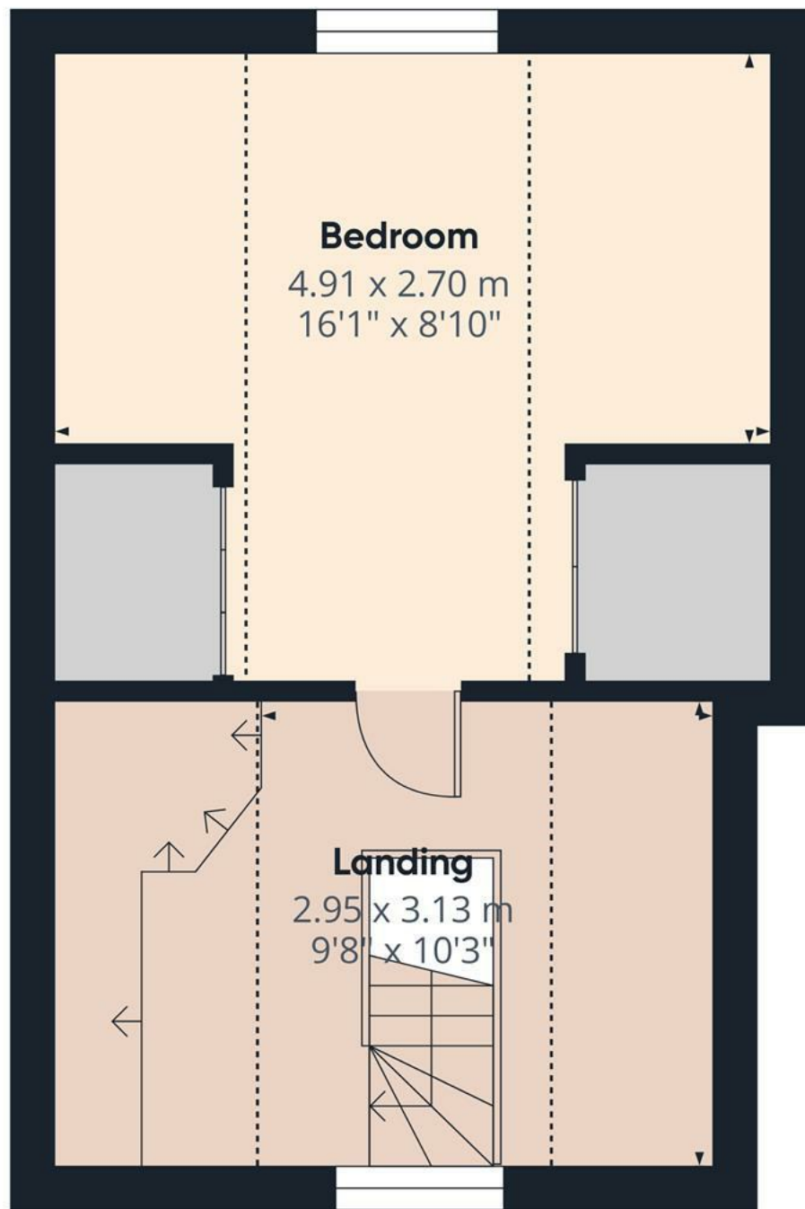
Floor 1
