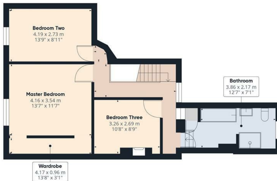
Floor 1 Building 1
